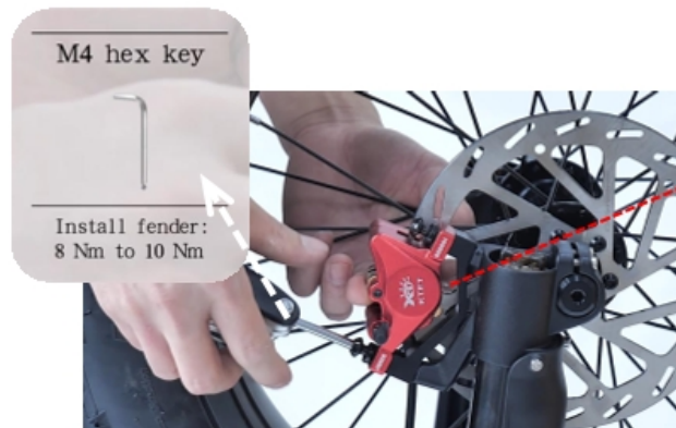
04 Tighten the screw
