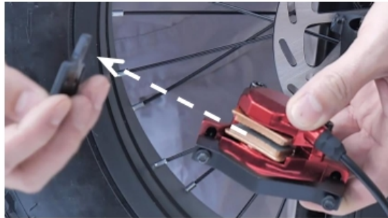
01 Remove the washer
